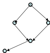
Layered graph
