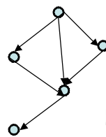
Directed graph
